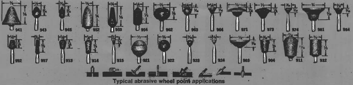
Typical abrasive wheel point applications
