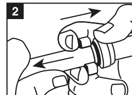
2. Place tool around pipe next to fitting. Press tool toward fitting while pulling pipe from fitting.
