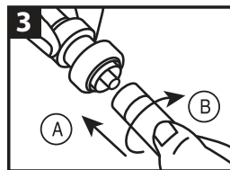
3. Push pipe (A) and twist (B) into fitting until fitting edge meets insertion line.
